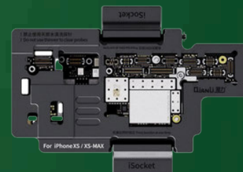
ISOCKET MEGA IDEA iPhone X - XS Max
