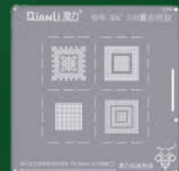
REBALLING STENCIL MAC-SSD QS92
