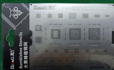
REBALLING STENCIL Qianli K50 QS210
