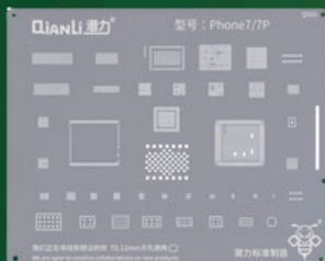
REBALLING STENCIL CPU & IC QS03
